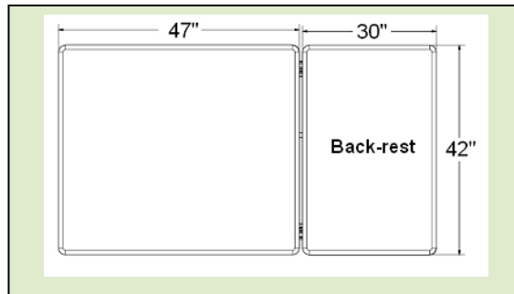
Mechanical back rest Block-O-Lift
